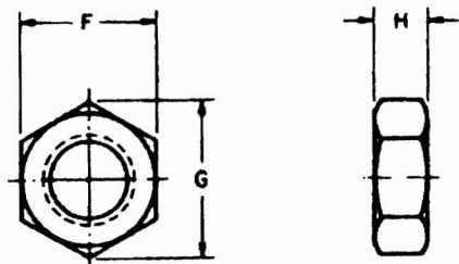
Hex Jam Nut, double-chamfered
