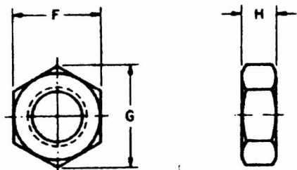
Heavy Hex Jam Nut, washer-faced and double-chamfered
